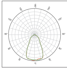
KFLEX4802A Symmetric beam 60° FWHM
