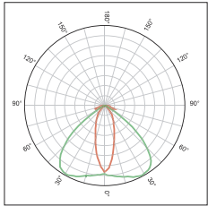
KFLEX6404A Elliptical beam 30°x100° FWHM
