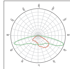
KFLEX3209A IESNA Type III Medium
