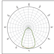
KFLEX1602A Symmetric beam 60°FWHM
