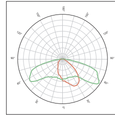
KFLEX4806A ECE M class narrow street
