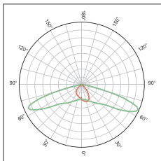
KFLEX1607A IESNA Type I Medium
