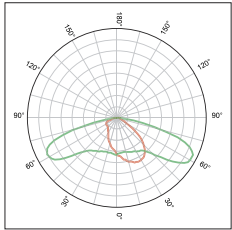
KFLEX3255B ECE M class
