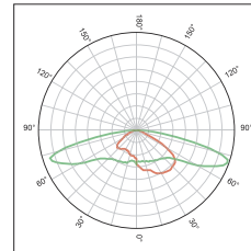
KFLEX6409A IESNA Type III Medium
