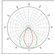
KFLEX6453B Elliptical beam 55°x95° FWHM
