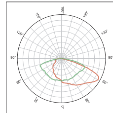
KFLEX3261B Vertical asymmetric beam
