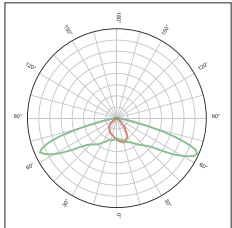
KFLEX3207A IESNA Type I Medium
