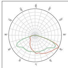
KFLEX3260B Vertical asymmetric beam
