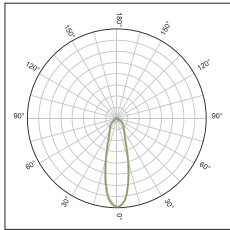
KFLEX1601A Symmetric beam 30°FWHM
