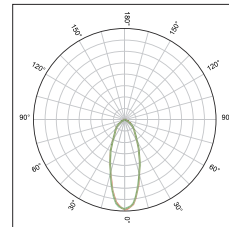
KFLEX3250B Symmetric beam 40°FWHM
