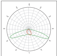
KFLEX6407A IESNA Type I Medium
