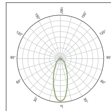
KFLEX6450B Symmetric beam 40°FWHM
