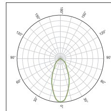
KFLEX4850B Symmetric beam 45°FWHM
