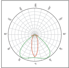
KFLEX3204A Elliptical beam 30°x100° FWHM
