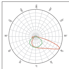
KFLEX4811A Vertical asymmetric beam for sports light
