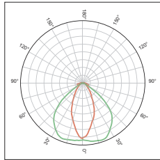
KFLEX4853B Elliptical beam 45°x100° FWHM
