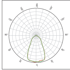
KFLEX3202A Symmetric beam 60° FWHM
