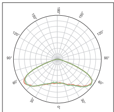
KFLEX4810A IESNA Type Vs Short
