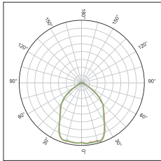
KFLEX6451B Symmetric beam 90°FWHM
