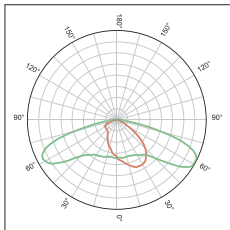
KFLEX6455B ECE M class
