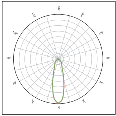
KFLEX4801A Symmetric beam 30°FWHM
