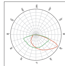
KFLEX6461B Vertical asymmetric beam
