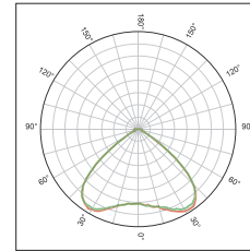
KFLEX1603A Symmetric beam 90°FWHM
