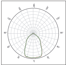
KFLEX4851B Symmetric beam 70°FWHM
