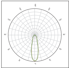
KFLEX6401A Symmetric beam 30°FWHM
