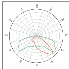
KFLEX1605A ECE M class wide street
