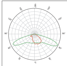
KFLEX3208A IESNA Type II Medium
