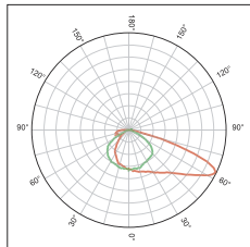
KFLEX3211A Vertical asymmetric beam for sports light
