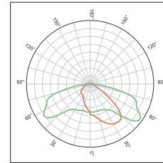
KFLEX6454B ECE M class
