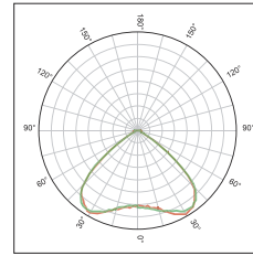
KFLEX4803A Symmetric beam 90° FWHM
