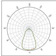
KFLEX6402A Symmetric beam 60°FWHM
