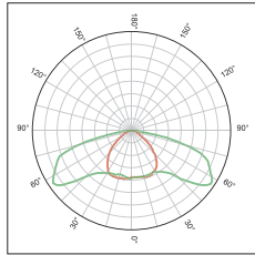
KFLEX3256B ECE M class on median installation
