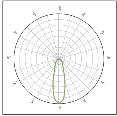
KFLEX3201A Symmetric beam 30°FWHM
