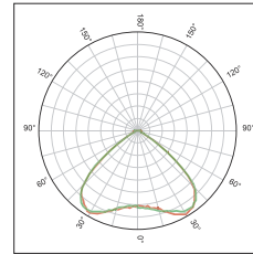
KFLEX6403A Symmetric beam 90°FWHM
