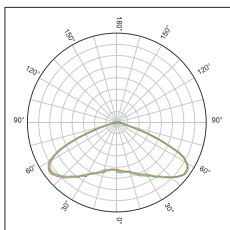
KFLEX1610A IESNA Type Vs Short
