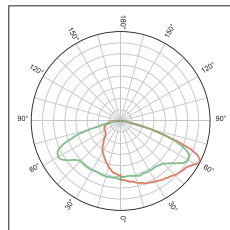
KFLEX6460B Vertical asymmetric beam
