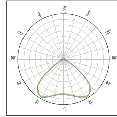
KFLEX3203A Symmetric beam 90° FWHM
