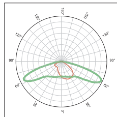
KFLEX1608A IESNA Type II Medium
