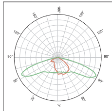
KFLEX6408A IESNA Type II Medium
