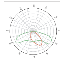
KFLEX1606A ECE M class narrow street
