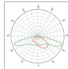
KFLEX1609A IESNA Type III Medium
