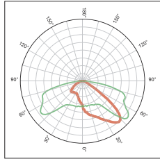
KFLEX3205A ECE M class wide street
