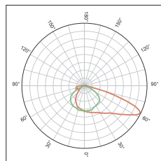
KFLEX1611A Vertical asymmetric beam for sports light
