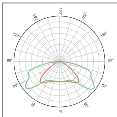
KFLEX6458B ECE M class on median installation
