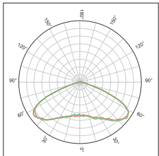
KFLEX3210A IESNA Type Vs Short
