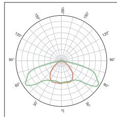
KFLEX6456B ECE M class on median installation
