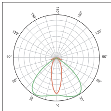
KFLEX1604A Elliptical beam 30°x100° FWHM
