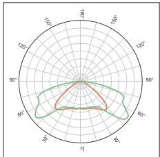
KFLEX3258B ECE M Class on median installation
