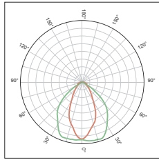
KFLEX3253B Elliptical beam 55°x95° FWHM
