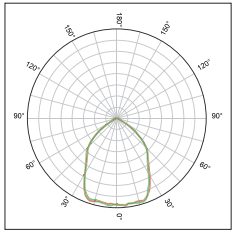
KFLEX3251B Symmetric beam 90°FWHM
