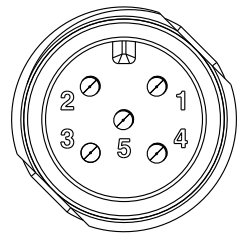
Conn. 4 Pin Assignments Front View
