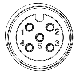
Conn. 1&2&3 Pin Assignments Front View
