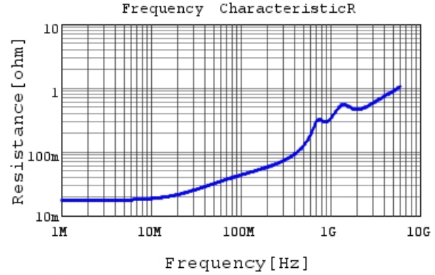
GRM2165C1H102JA01 R DCOV,25degC
