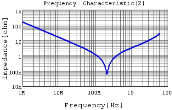
GRM2165C1H102JA01 |Z| DCOV,25degC
