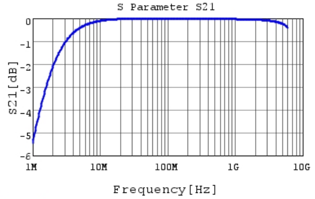
GRM2165C1H102JA01 S21 DCOV, 25degC
