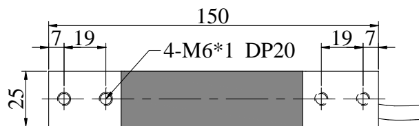
俯視(Top View)
