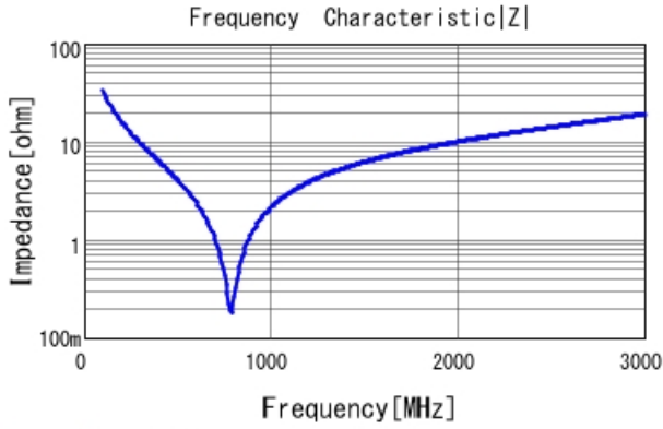
GRM31A5C3A470JW01 |Z| DCOV, 25degC
