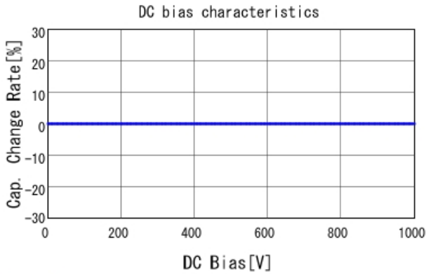
GRM31A5C3A470JW01 C-DC bias capchange, 25.0degC, A
