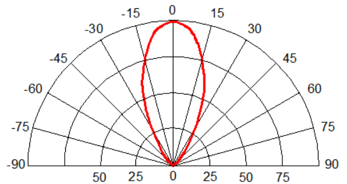
Fig.8 Radiation pattern@30mA
