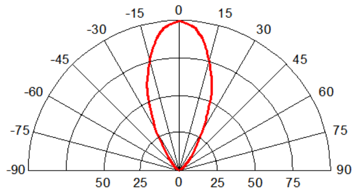
Fig.8 Radiation pattern@350mA
