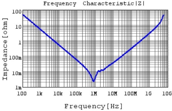
GRM32ER71A476KE15 |Z| DCOV,25degC
