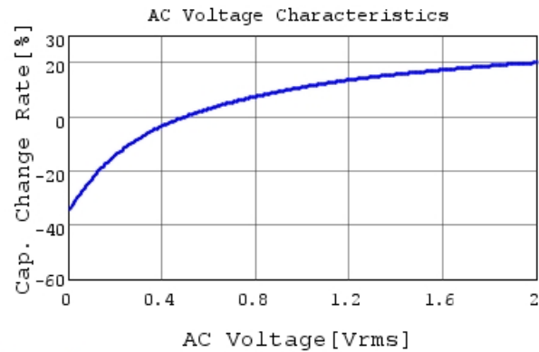
GRM32ER71A476KE15 C-AC Voltage capchange, Dc
