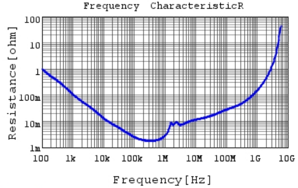
GRM32ER71A476KE15 R DCOV,25degC
