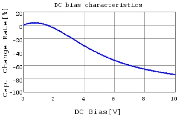
GRM32ER71A476KE15 C-DC bias capchange, 25.0c
