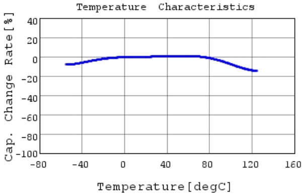
GRM32ER71A476KE15 C-Temp. capchange, DC0.0V,
