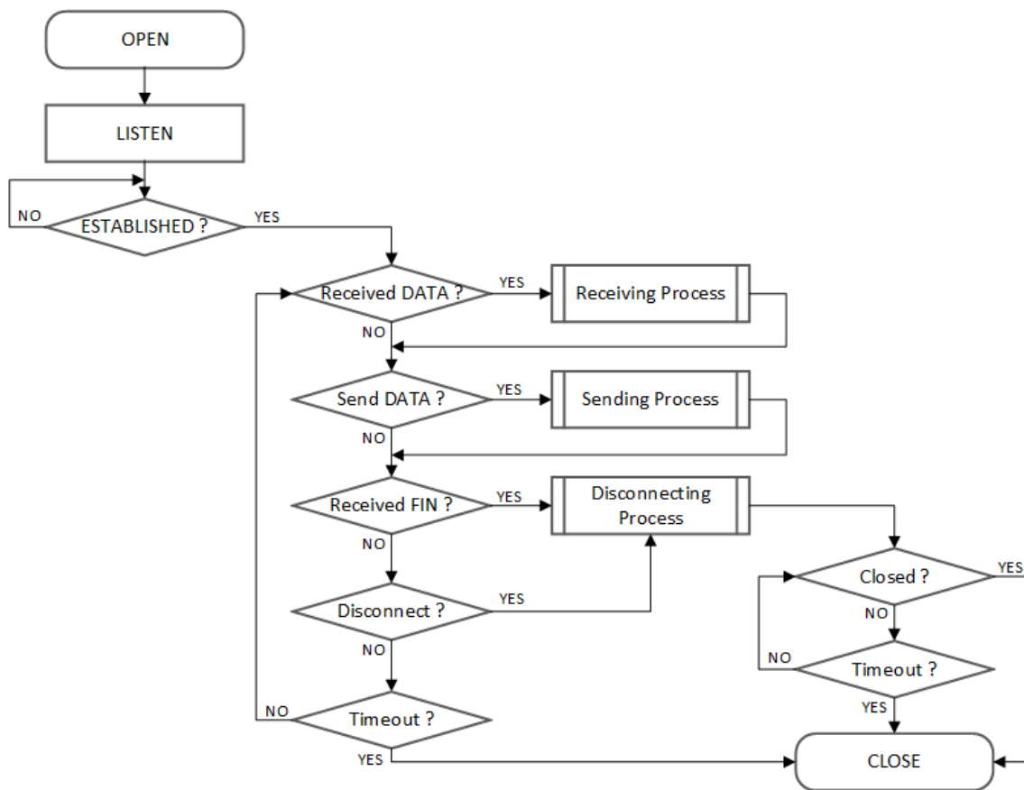
Figure 6 TCP Server Operation Flow
