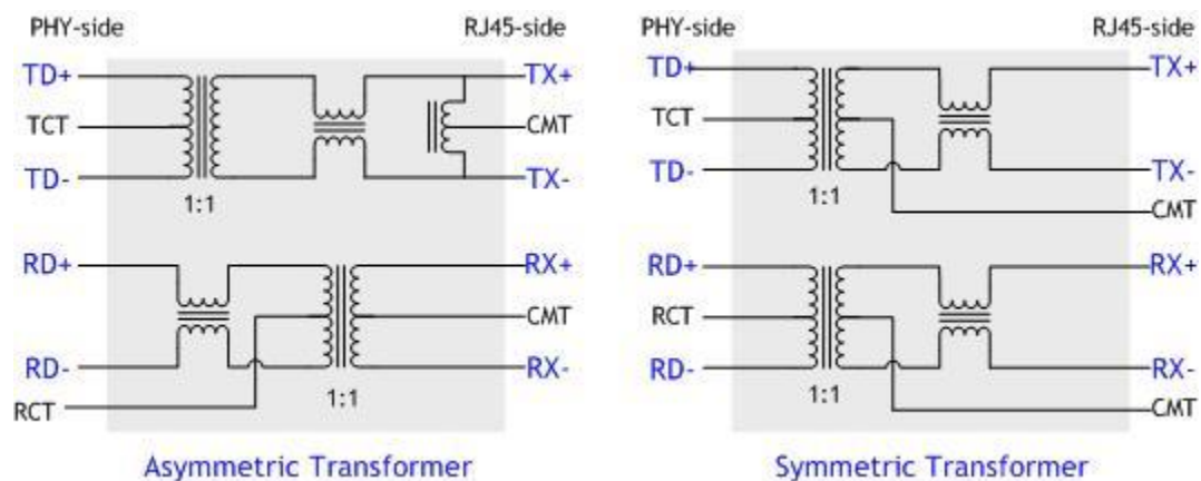
Figure 30 Transformer Type
