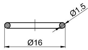
Seal Ring
