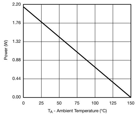
Power, Junction-to-Ambient
