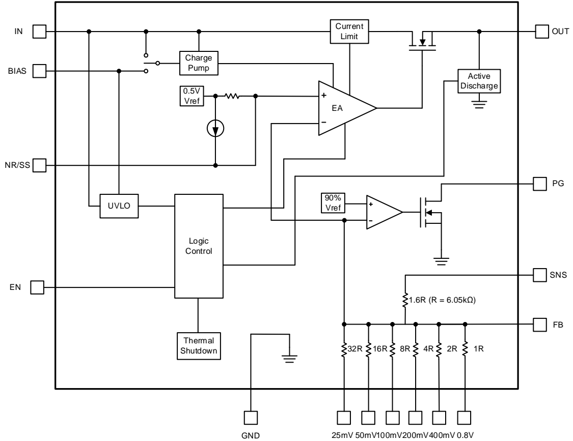
Figure 4-1 Block diagram for GD30LD3300x
