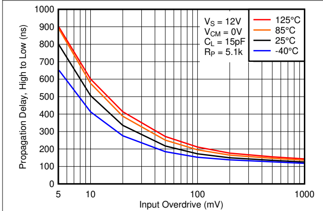
Figure 7-27. High to Low Propagation Delay vs. Input Overdrive Voltage, 12V
