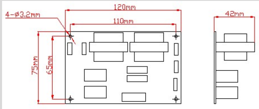
Installation Dimension
