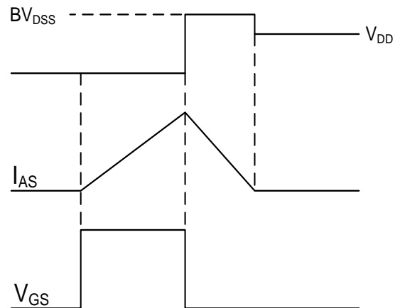
Fig.11 EAS Waveform
