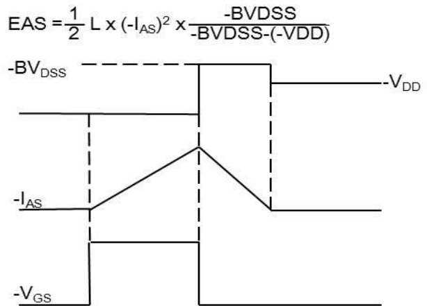
Fig.10 EAS Waveform
