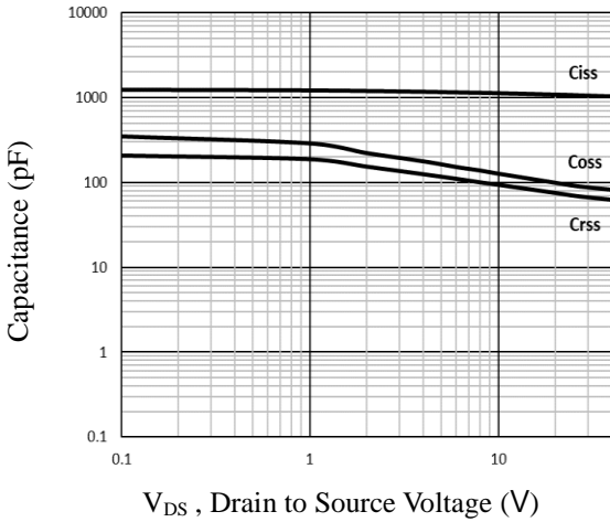
Fig.7 Capacitance Characteristics
