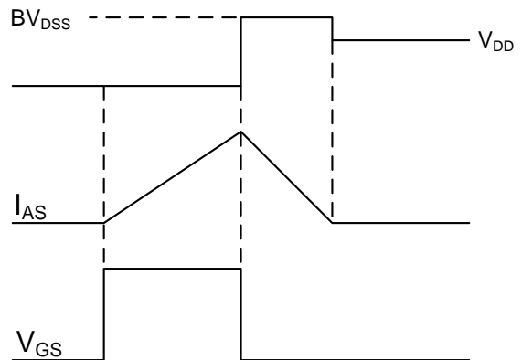
Fig.11 EAS Waveform
