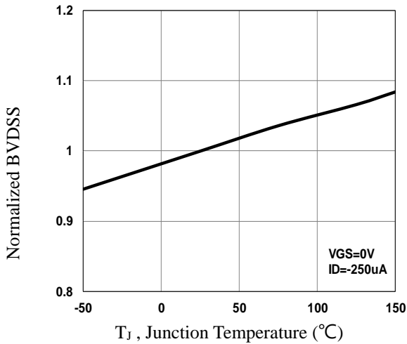
Fig.21 Normalized BVDSS vs. T J
