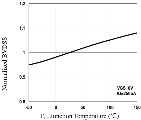
Fig.9 Normalized BVDSS vs. T J
