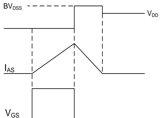
Fig.11 EAS Waveform
