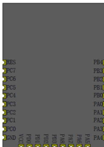
Figure 3 Bottom View
