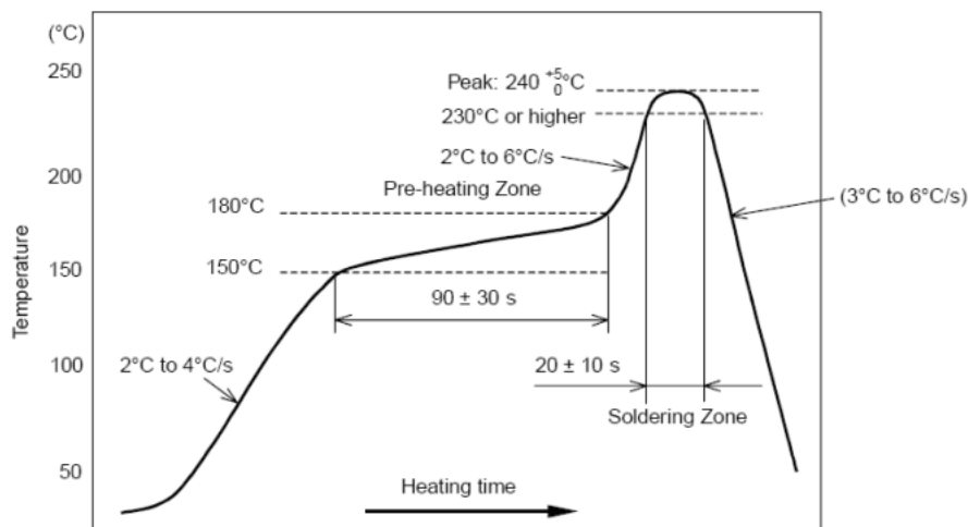
Fig. 8 Welding heat resistance temperature curve of components (welding points)
