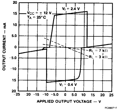
Typical Output Current vs Applied Output Voltage
