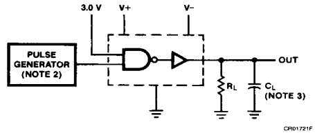
Figure 6 Switching Characteristics
