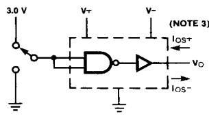
Figure 4 I_{OS}
