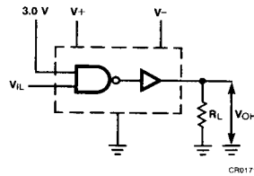
Figure 4 I_{OS}
