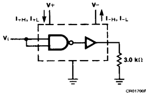
Figure 5 I_{+H} , I_{-H} , I_{+L} , I_{-L} (Note 1)
