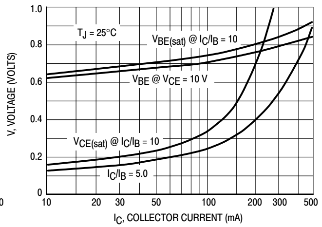
Figure 2. "On" Voltages
