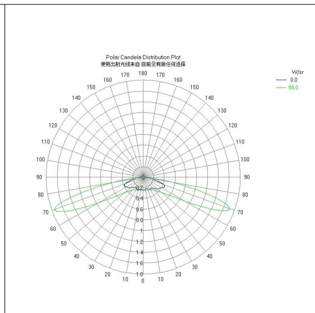
Optical simulation
