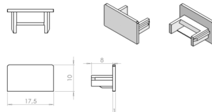
Endcap
