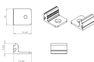
Holder-R
